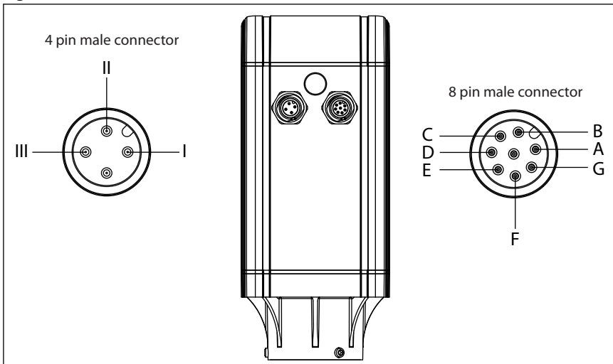
Figure 5: Connector
