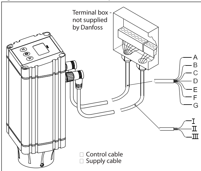
Figure 5: Connector
