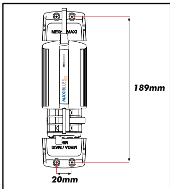
PUMP FITTED WITH MOUNTING FEET
